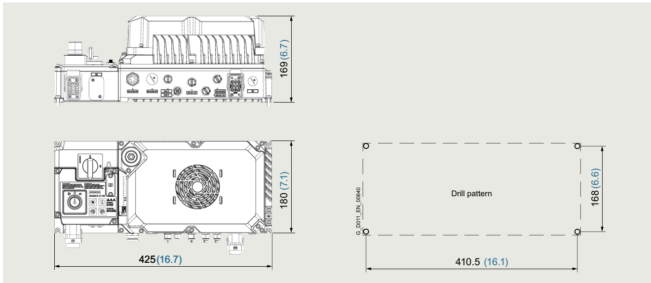
SINAMICS G115D frame size FSC, with fan
