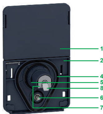
Remote-mounting kit for mounting graphic display terminal (rear face)
