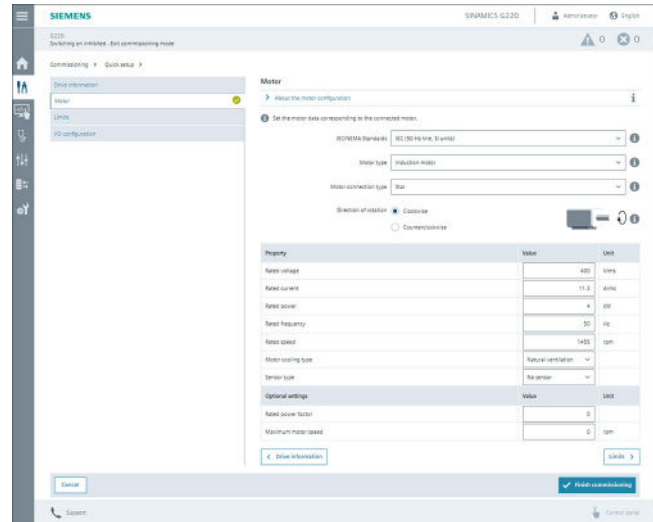
Quick commissioning with open dialog showing the set motor data
