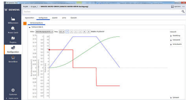
Dimensioning – Traversing profile editor with graphical and tabular input
