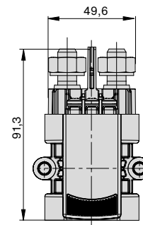
MPR10/MPR20 Dimensional drawing
