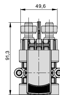
HPR10 Dimensional drawing
