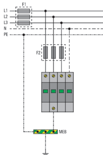
Fuse protection of SPDs
