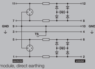
Complete module, direct earthing
