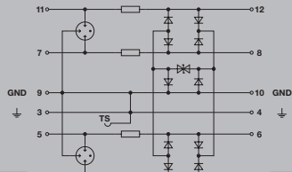
Complete module, direct earthing
