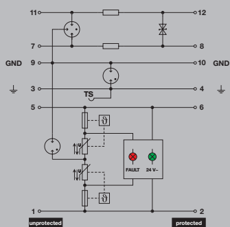
Complete module, indirect earthing
