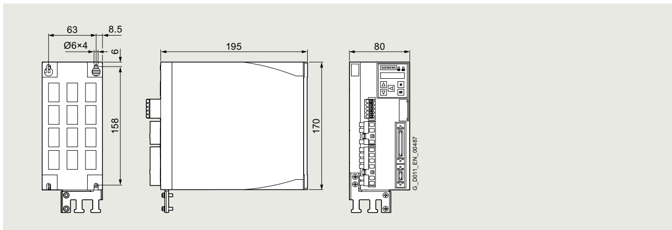
SINAMICS V90, 200 ... 240 V 1 AC/3 AC, frame size FSC
