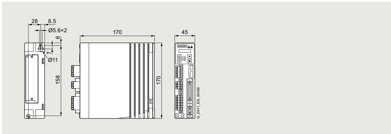
SINAMICS V90, 200 ... 240 V 1 AC/3 AC, frame size FSA
