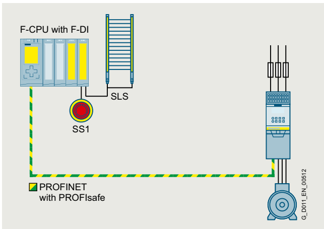
Integrated safety solution via PROFINsafe
