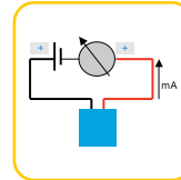
Passive Current
