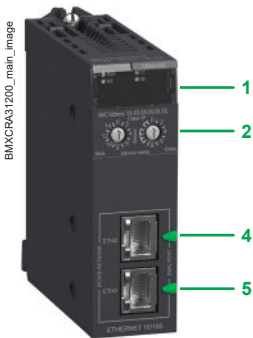
BMXCRA31200
