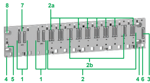
BMEXBP1002 backplane
