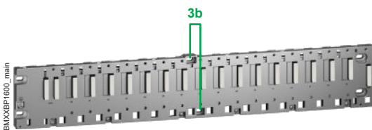
BMXXBP1600 with 16 slots and additional fixing holes
