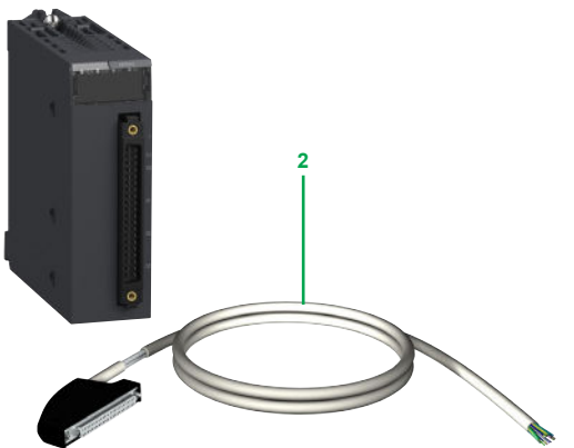
BMXFCW01S cordset (with 40-way connector at one end and flying leads at the other)
