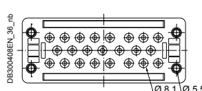
KDP 24/23
