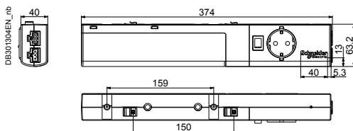
Magnetic Fixing
