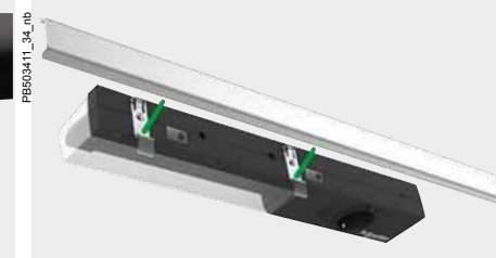
Fixing to DIN Rail
