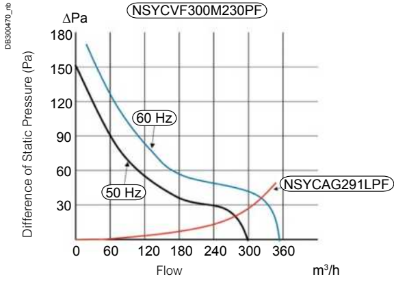
Flow Curves
