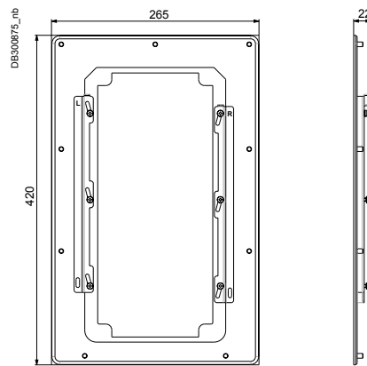
NSYPTDS2
