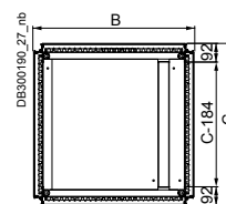
Enclosures of 300 and 400 mm width.
