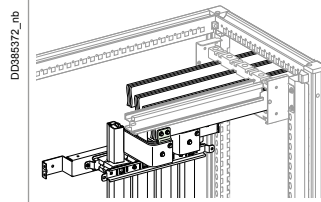
LVS04635 Connection to 5 mm Thick Horizontal Busbar
