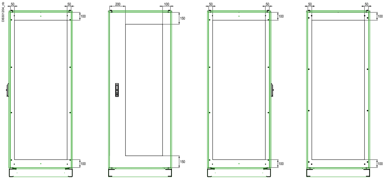
Cut-Outs
