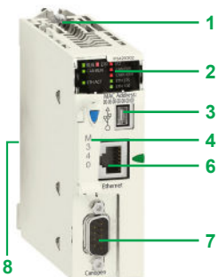
BMXP3420302/BMXP3420302CL
