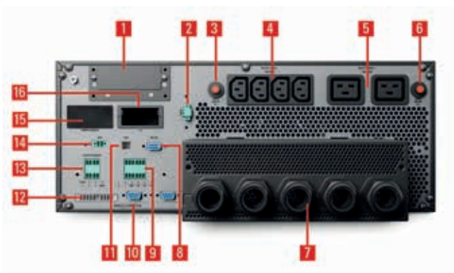
SLC-7,5-20-CUBE4 R
