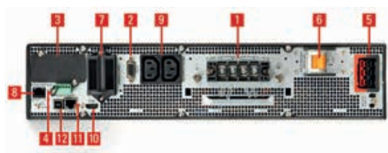
SLC 4000÷10000 TWIN RT3
