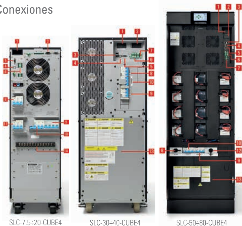
SLC-7,5-20-CUBE4
