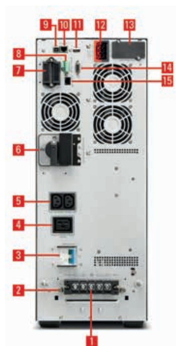
SLC 4000-10000 TWIN PRO3
