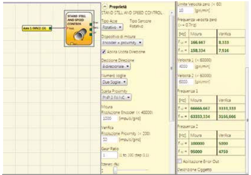
Speed monitoring object configuration example
