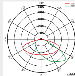
VA00I0P (≤900mA)
