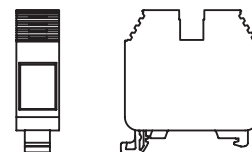
Borne 4 / 10 / 16 / 35
