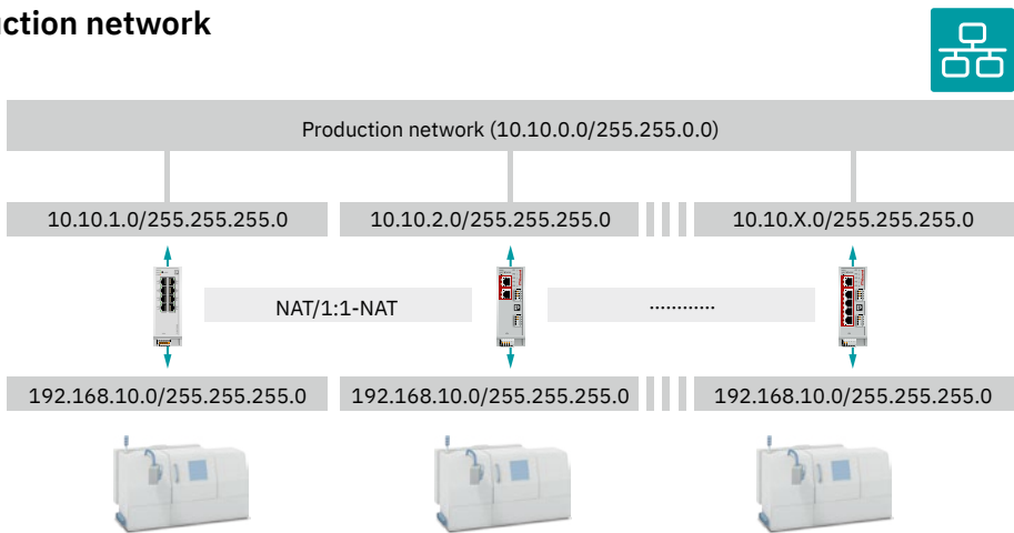
Machine connection with NAT and security routers
