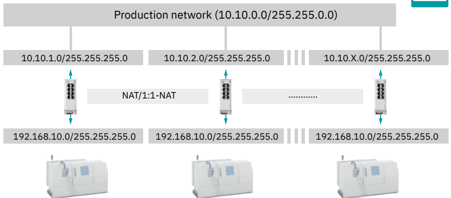
Automatic IP address translation using switches with NAT function
