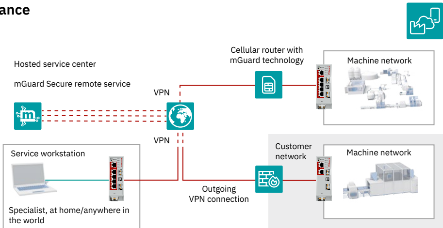
Secure remote maintenance concept with mGuard components
