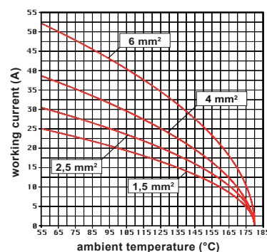
CP RY 06 inserts max. current load derating diagram
