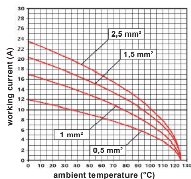
JSH 10 inserts max. current load derating diagram
