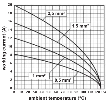
CQ 17 inserts max. current load derating diagram, turned contacts
