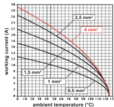
CMCE 10 inserts max. current load derating diagram
