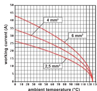
RX 12/2 inserts max. current load derating diagram
