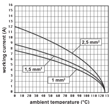
CD 40 inserts max. current load derating diagram, turned contacts
