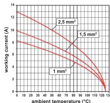
CX 42 D inserts max. current load derating diagram
