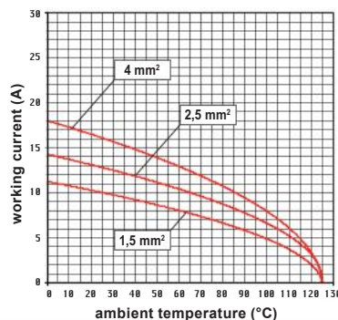
RQEE 64 inserts max. current load derating diagram
