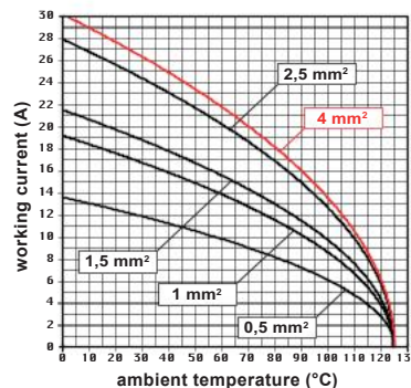
CNE 06 T inserts max. current load derating diagram
