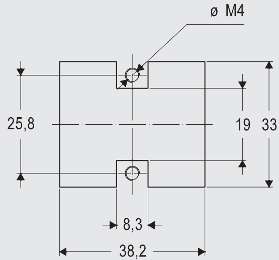
MIXO TWO bulkhead mounting housings threaded panel
