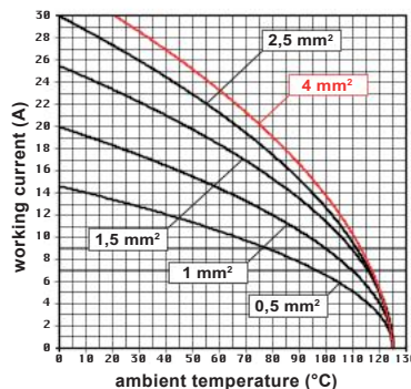
CMSH 06 inserts max. current load derating diagram
