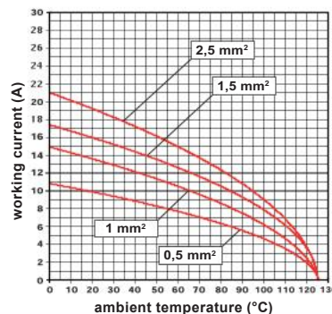
JSH 16 inserts max. current load derating diagram
