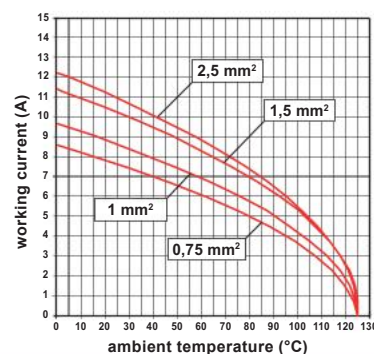
CX 12 D inserts max. current load derating diagram
