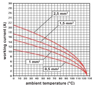
RSH 16 inserts max. current load derating diagram
