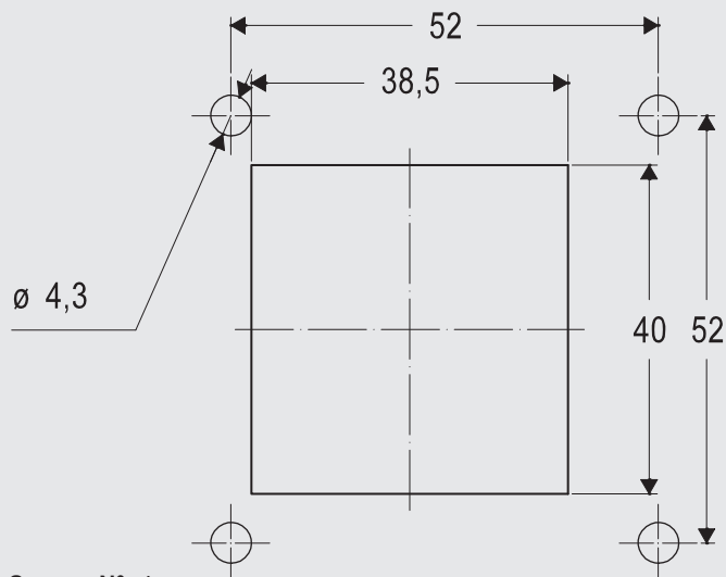
MIXO TWO angled bulkhead mounting housings through-holes panel
