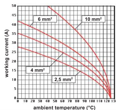
CX 03 4B inserts max. current load derating diagram
