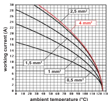
CMSH 03 inserts max. current load derating diagram
