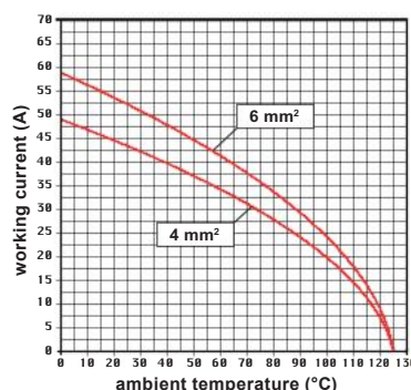
CX 6/36 inserts max. current load derating diagram
