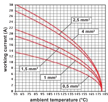
CNE 06 RY inserts max. current load derating diagram
