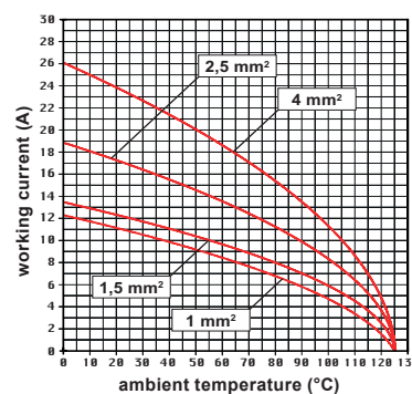
CX 8/24 inserts max. current load derating diagram, power poles
