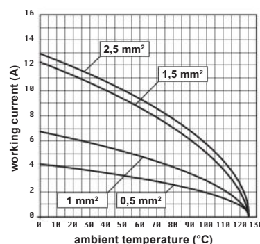
CDD 42 inserts max. current load derating diagram, turned contacts
