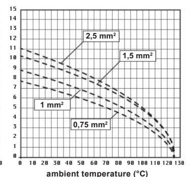
CX 12 D inserts max. current load derating diagram, stamped contacts
