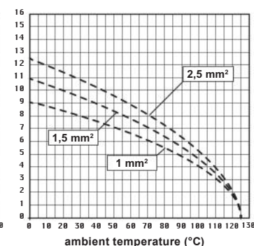
CD 25 inserts max. current load derating diagram, stamped contacts
