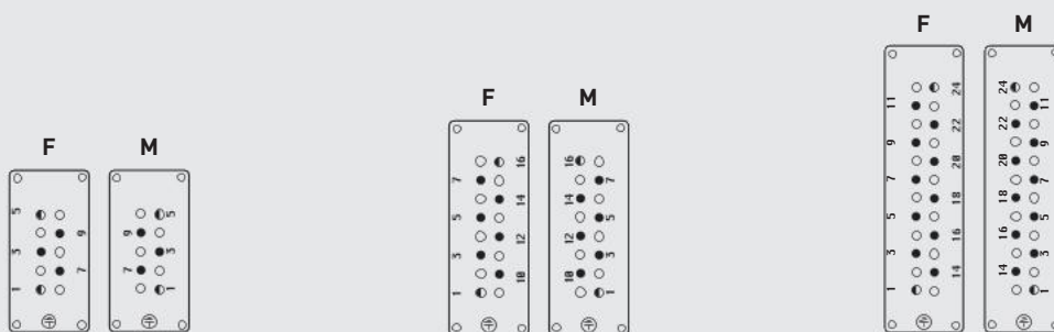
contacts side - front view
