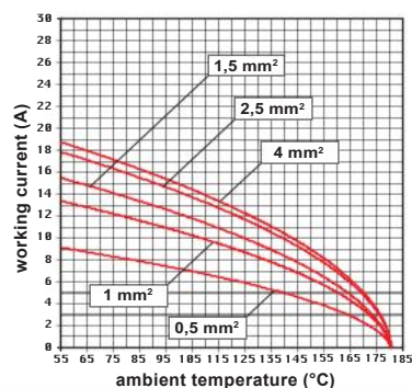
CNE 24 RY inserts max. current load derating diagram
