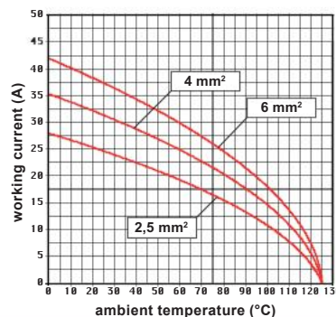
CX 03 4 inserts max. current load derating diagram
