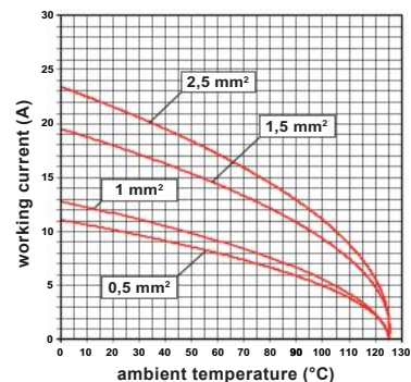
RDSH 09 inserts max. current load derating diagram
