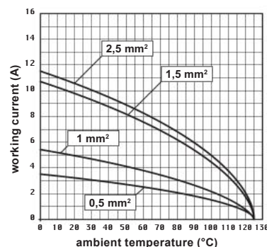
CDD 72 inserts max. current load derating diagram, turned contacts
