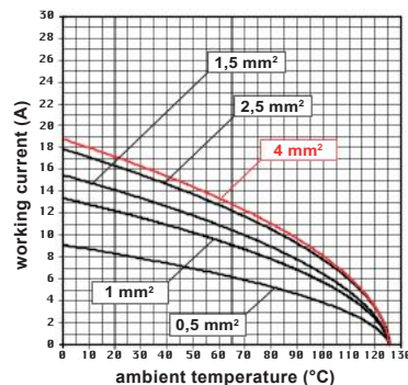
RCE 24 inserts max. current load derating diagram
