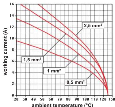
CT 16 inserts max. current load derating diagram
