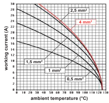
CMCE 03 inserts max. current load derating diagram
