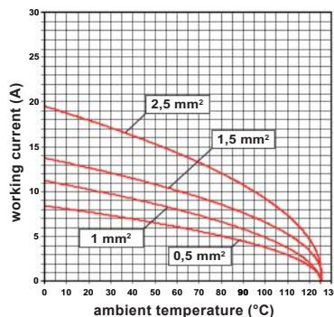
CDSH 27 inserts max. current load derating diagram
