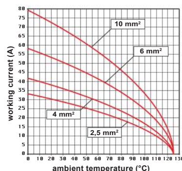
CQ 04/2B inserts max. current load derating diagram
