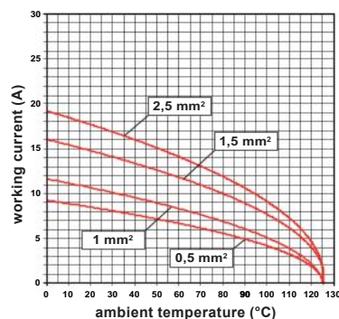
CDSH 18 inserts max. current load derating diagram
