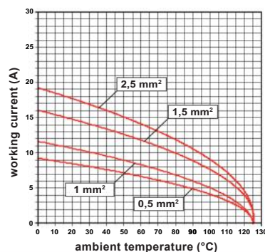
RDSH 18 inserts max. current load derating diagram
