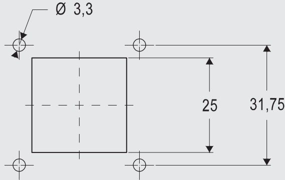
Size 21.21 fixing by 4 screws
