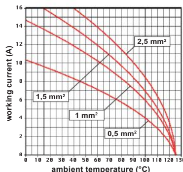
CTSE 24 inserts max. current load derating diagram
