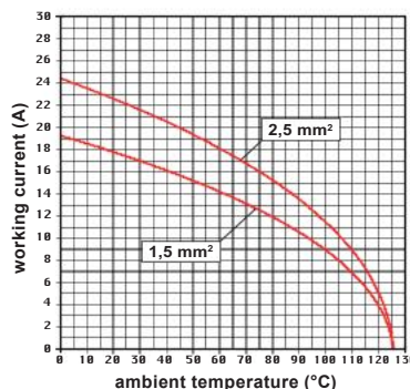
CSS 06 inserts max. current load derating diagram
