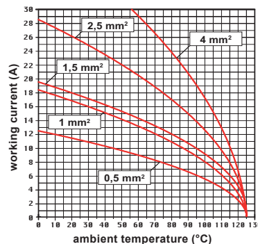
RQ 05 inserts max. current load derating diagram
