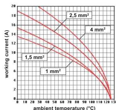
CX 06P C inserts max. current load derating diagram
