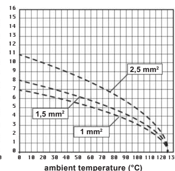
CD 40 inserts max. current load derating diagram, stamped contacts
