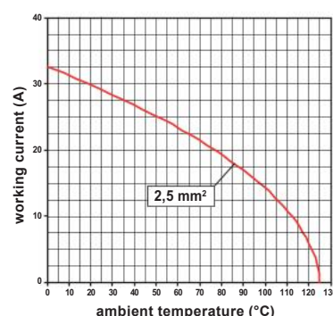
CX 02 CH inserts max. current load derating diagram
