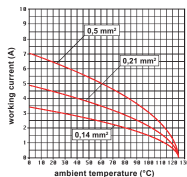
CQ 21 inserts max. current load derating diagram
