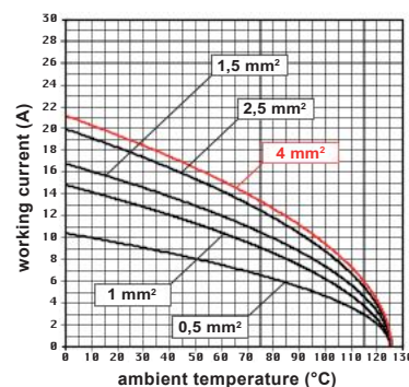
RCE 16 inserts max. current load derating diagram
