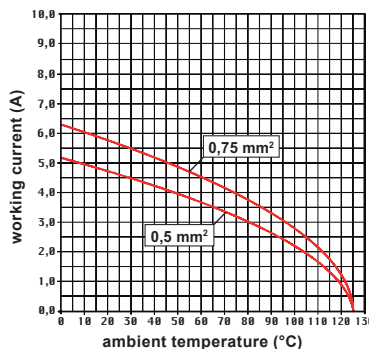
CX 25 IB inserts max. current load derating diagram
