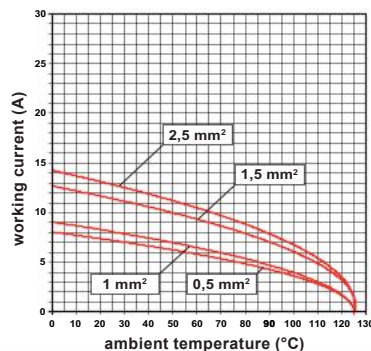
RDSH 42 inserts max. current load derating diagram
