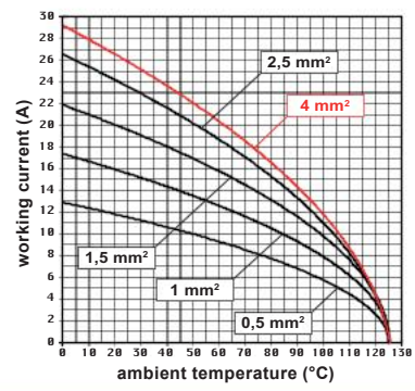
CMCE 10 inserts max. current load derating diagram
