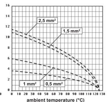
CDD 42 inserts max. current load derating diagram, stamped contacts
