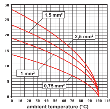
JK 04 inserts max. current load derating diagram
