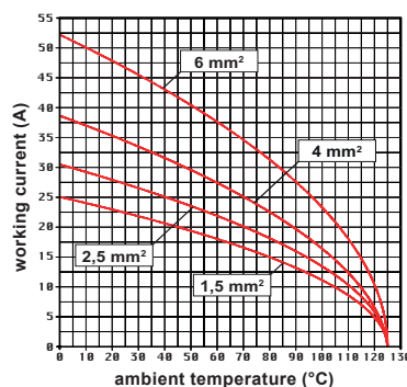
CP 06 inserts max. current load derating diagram
