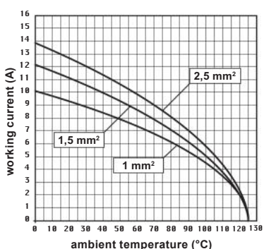
CD 25 inserts max. current load derating diagram, turned contacts
