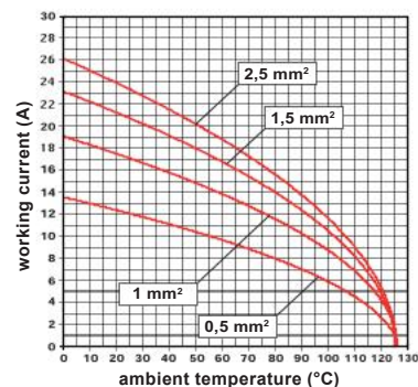
RSH 06 inserts max. current load derating diagram
