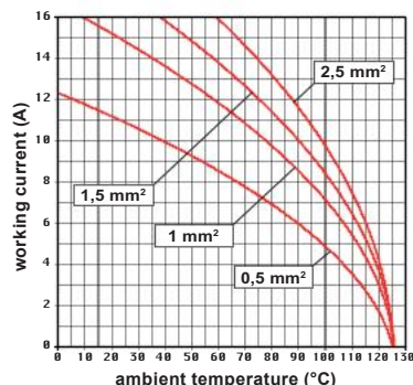
CTSE 10 inserts max. current load derating diagram
