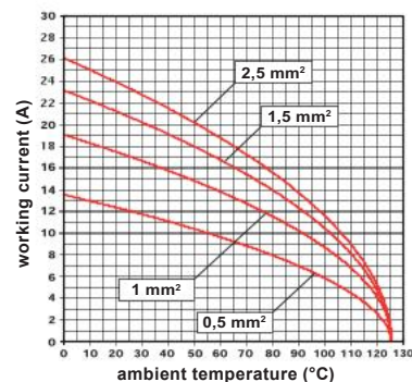
JSH 06 inserts max. current load derating diagram
