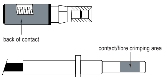
Fig. 4 - Female contact/fibre crimping area
