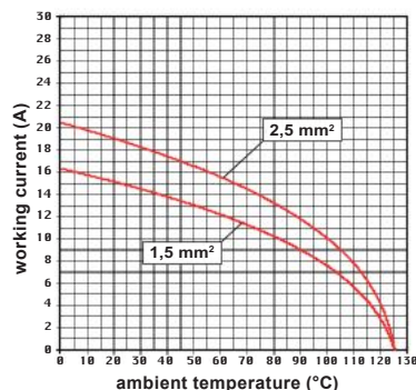
CSS 10 inserts max. current load derating diagram
