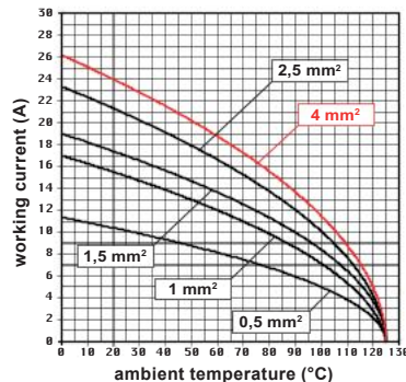
RCE 10 inserts max. current load derating diagram
