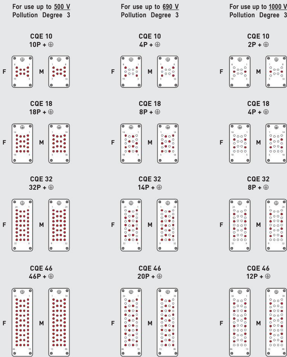
contacts side - front view
