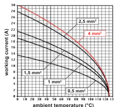
CCE 06 inserts max. current load derating diagram
