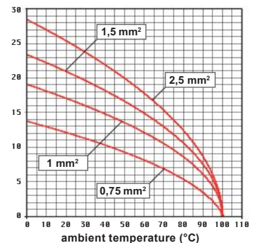
CKSH 04 inserts max. current load derating diagram
