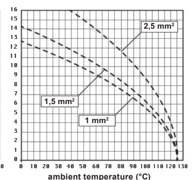
CD 07 inserts max. current load derating diagram, stamped contacts
