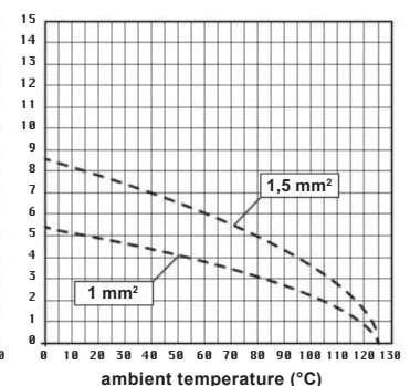
CX 17 D inserts max. current load derating diagram, stamped contacts
