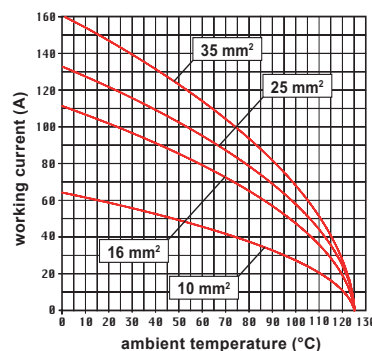
CX 6/6 inserts max. current load derating diagram
