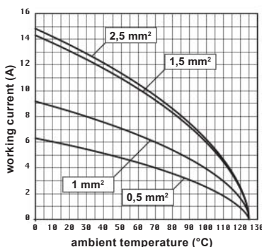
CDD 24 inserts max. current load derating diagram, turned contacts
