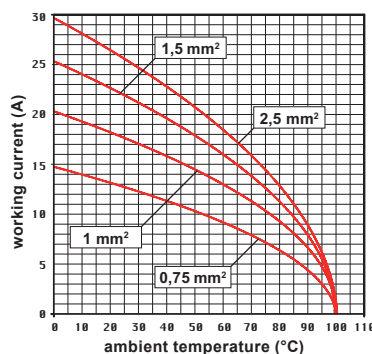
JK 03 inserts max. current load derating diagram
