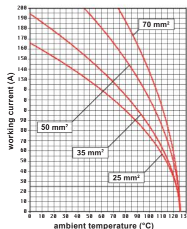
CX 01 YA inserts max. current load derating diagram
