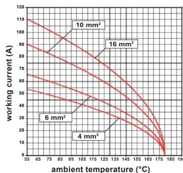
CX 4/0 RY inserts max. current load derating diagram
