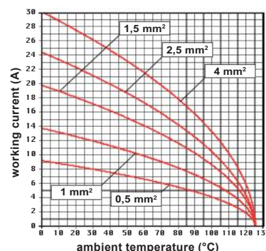
CQE 10 inserts max. current load derating diagram
