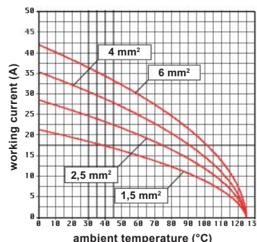
CX 3/4 XD inserts max. current load derating diagram
