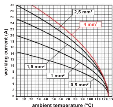
CMCE 06 inserts max. current load derating diagram
