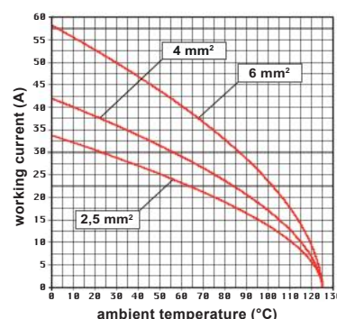
CQ 04/2E inserts max. current load derating diagram
