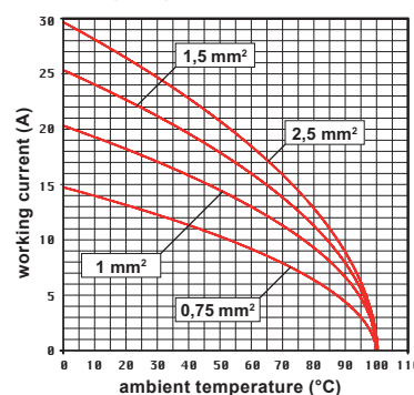
CKD 03 inserts max. current load derating diagram
