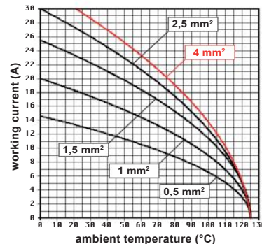
CMSH 06 inserts max. current load derating diagram
