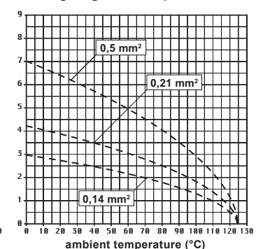
CQ 21 inserts max. current load derating diagram, stamped contacts
