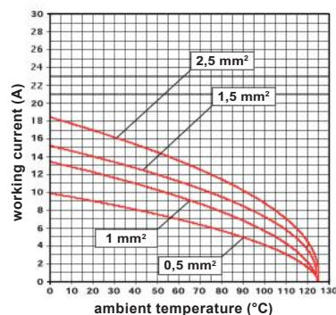
JSH 24 inserts max. current load derating diagram
