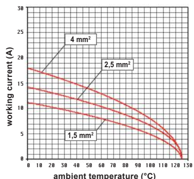
CQEE 64 inserts max. current load derating diagram
