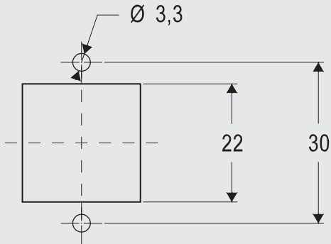
Size 21.21 fixing by 2 screws
