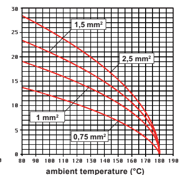
CK RY 04 inserts max. current load derating diagram
