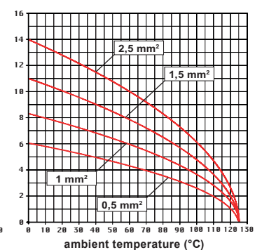
CX 8/24 inserts max. current load derating diagram, aux. poles
