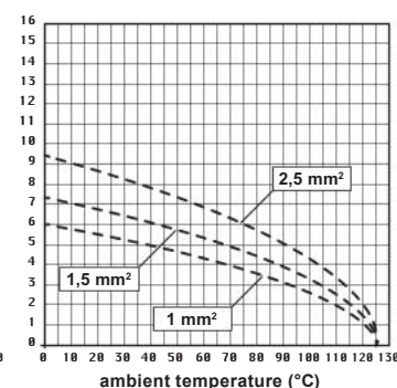
CD 64 inserts max. current load derating diagram, stamped contacts
