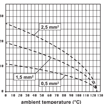
CQ 07 inserts max. current load derating diagram, stamped contacts
