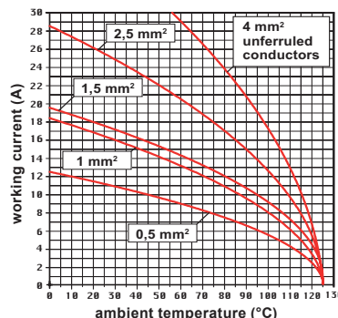
CQY 05 inserts max. current load derating diagram
