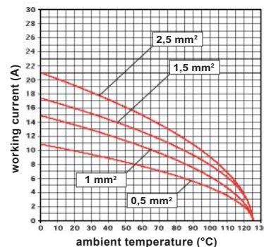
JSH 16 inserts max. current load derating diagram
