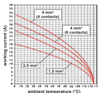
CQ 08 inserts max. current load derating diagram
