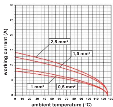
CDSH 42 inserts max. current load derating diagram
