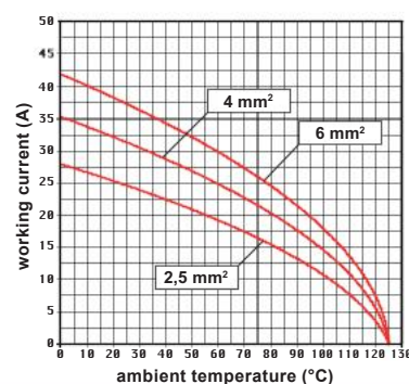
CX 03 4 inserts max. current load derating diagram
