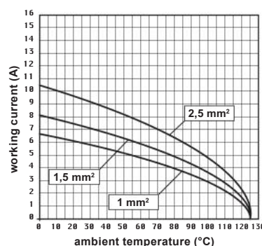
CD 64 inserts max. current load derating diagram, turned contacts
