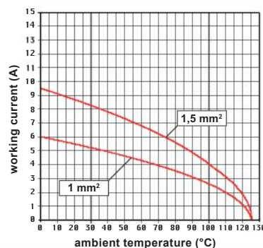
CX 17 D inserts max. current load derating diagram
