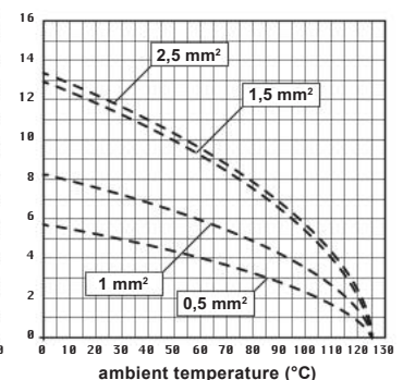
CDD 24 inserts max. current load derating diagram, stamped contacts
