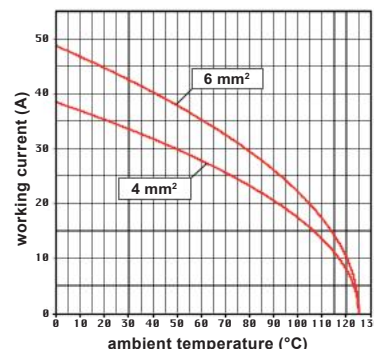
CX 9/42 inserts max. current load derating diagram
