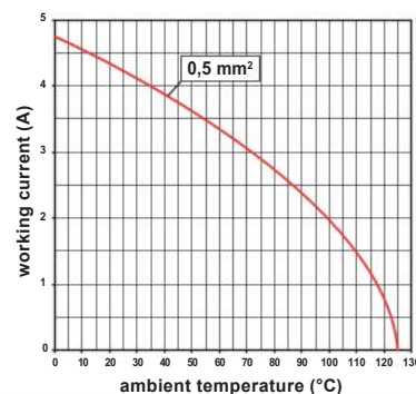
CX 36 I inserts max. current load derating diagram
