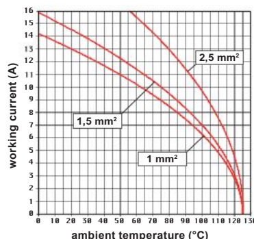
CD 08 inserts max. current load derating diagram
