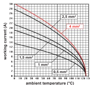
RCE 06 inserts max. current load derating diagram
