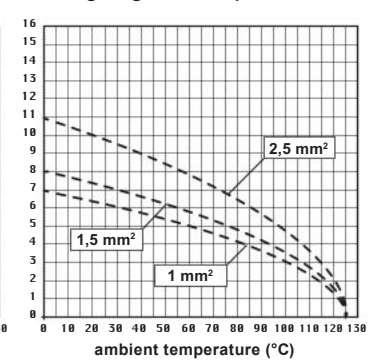
CD 40 inserts max. current load derating diagram, stamped contacts
