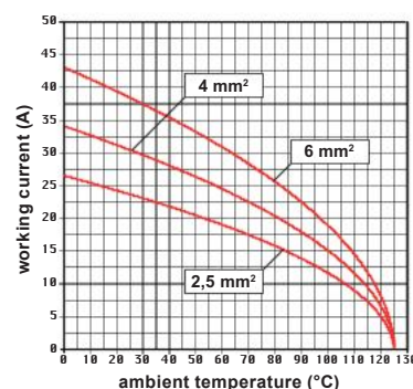
CX 12/2 inserts max. current load derating diagram
