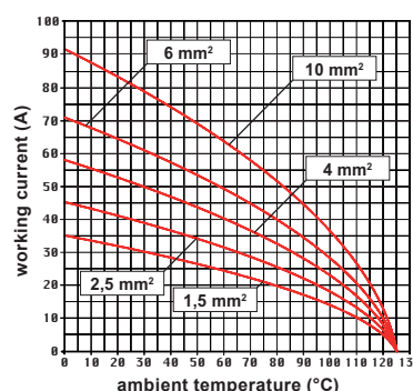
CQ4 02 inserts max. current load derating diagram
