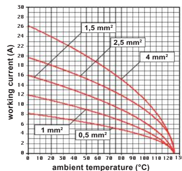
CQEY 18 inserts max. current load derating diagram
