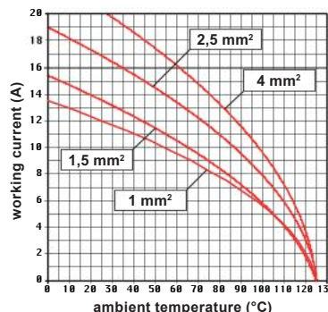
CX 06 C inserts max. current load derating diagram
