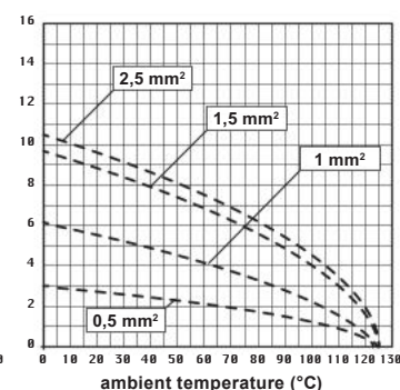
CDD 108 inserts max. current load derating diagram, stamped contacts
