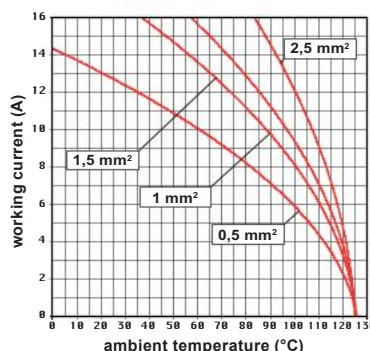
CTSE 06 inserts max. current load derating diagram
