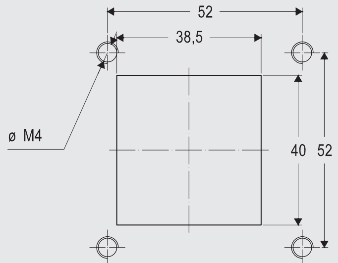
MIXO TWO angled bulkhead mounting housings threaded panel
