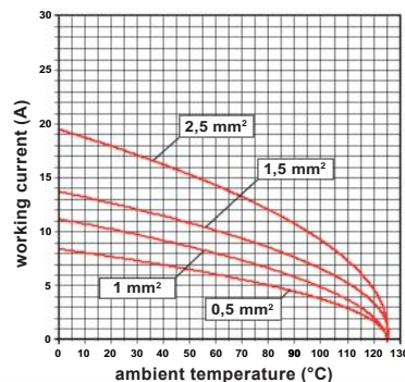
RDSH 27 inserts max. current load derating diagram
