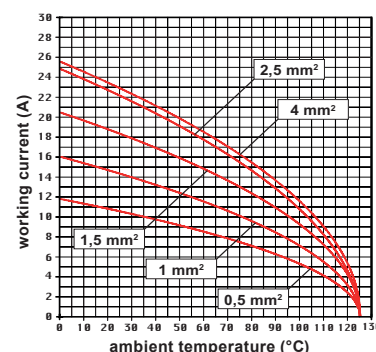
CDC 10 inserts max. current load derating diagram
