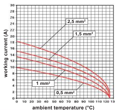
RSH 24 inserts max. current load derating diagram
