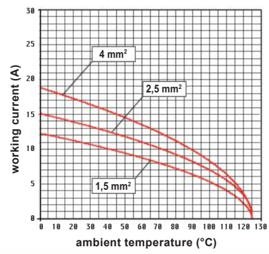
CQEE 40 inserts max. current load derating diagram
