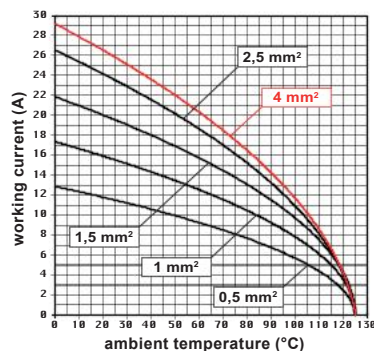
CMSh 10 inserts max. current load derating diagram
