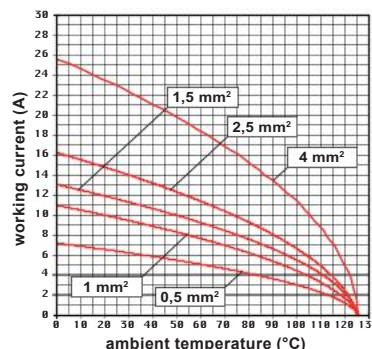
CQE 32 inserts max. current load derating diagram
