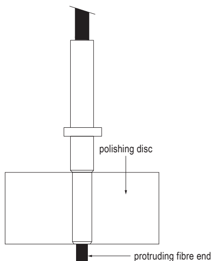
Fig. 6 - Polishing Disc with Guide for Connector Sleeve
