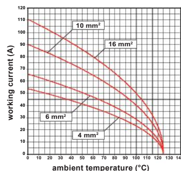
CX 4/0 inserts max. current load derating diagram
