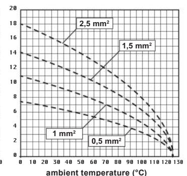
CQ 17 inserts max. current load derating diagram, stamped contacts
