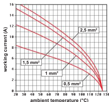
CT 24 inserts max. current load derating diagram
