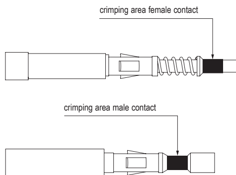
Fig. 4 - Crimping area
