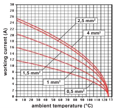
CDA 10 inserts max. current load derating diagram
