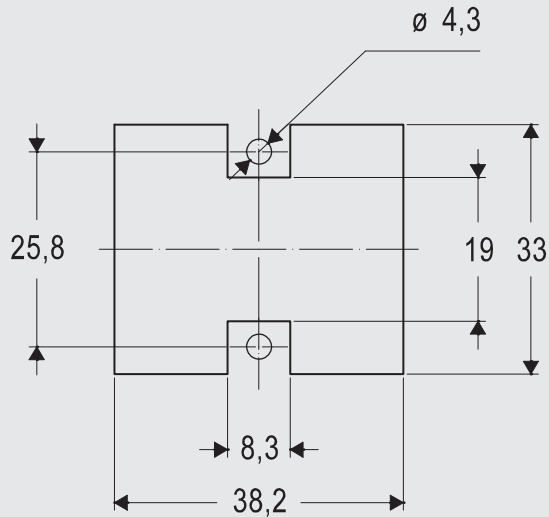
MIXO TWO bulkhead mounting housings through-holes panel (max. thickness: 6 mm)
