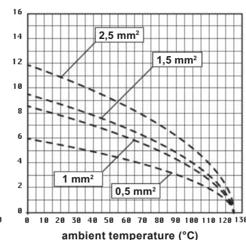
CDD 38 inserts max. current load derating diagram, stamped contacts
