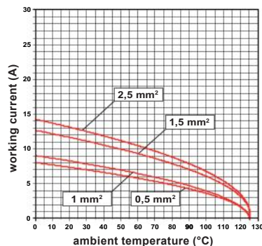
CDSH 42 inserts max. current load derating diagram
