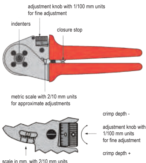
Fig. 5 (manual crimping tool)
