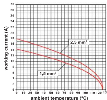
CSS 16 inserts max. current load derating diagram
