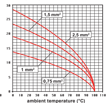
CKD 04 inserts max. current load derating diagram
