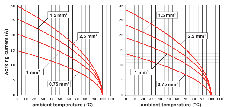
CK 03 inserts max. current load derating diagram
