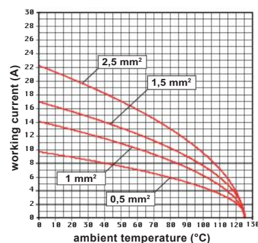
CSAH 16 inserts max. current load derating diagram
