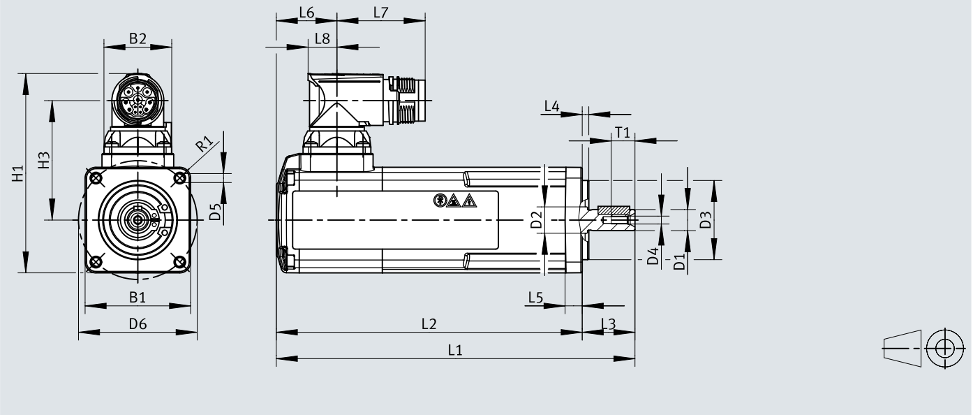
Dimensions – EMMT-EC-40
