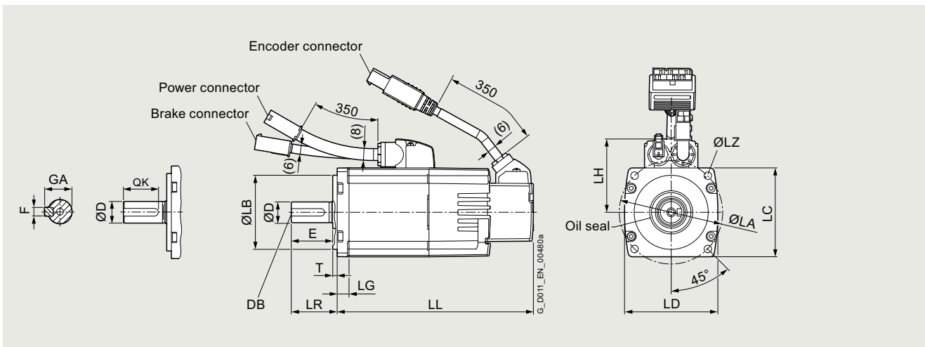
SIMOTICS S-1FL6 Low Inertia servomotors, shaft heights 20, 30, 40
