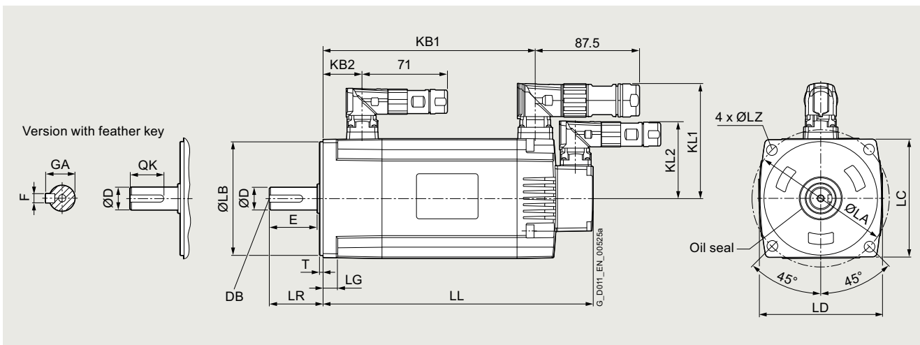
SIMOTICS S-1FL6 Low Inertia servomotor, shaft height 50
