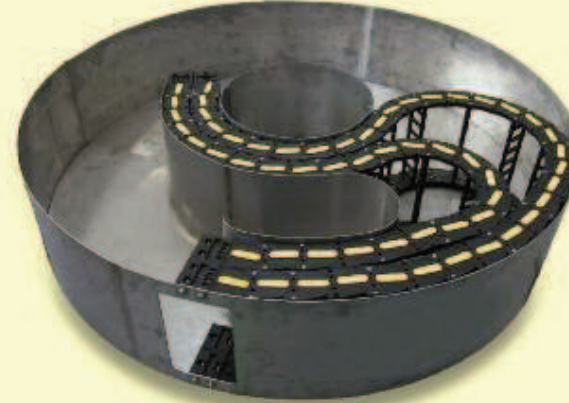
Application with 2 superimposed chains. Rotation 180°
