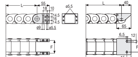
Fig. B Chain fixed outside the radius. (Fig B) See end brackets mounting variations page 31.
