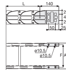
Fig. A The chain can be fixed frontally. See end brackets mounting variations page 31.
