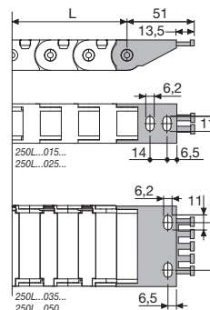
Fig. A Chain fixed outside the radius. (Fig A) See end brackets mounting variations page 31.
