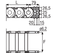
Fig. A The chain can be fixed frontally, inner or outer radius. (Fig A) See end brackets mounting variations page 31.
