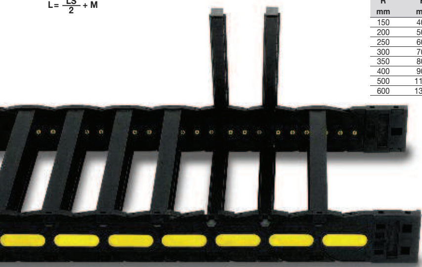
Version with frames mounted on every pitch.
