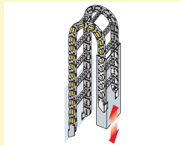
Vertical with curve above (see page 20).
