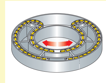
Chain for circular movement - 2 chains (see page 26).
