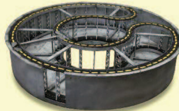
Application with 2 chains. Rotation 370°
