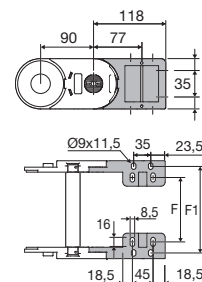
Fig. A The chain can be fixed frontally, inner and outer radius (Fig A)
