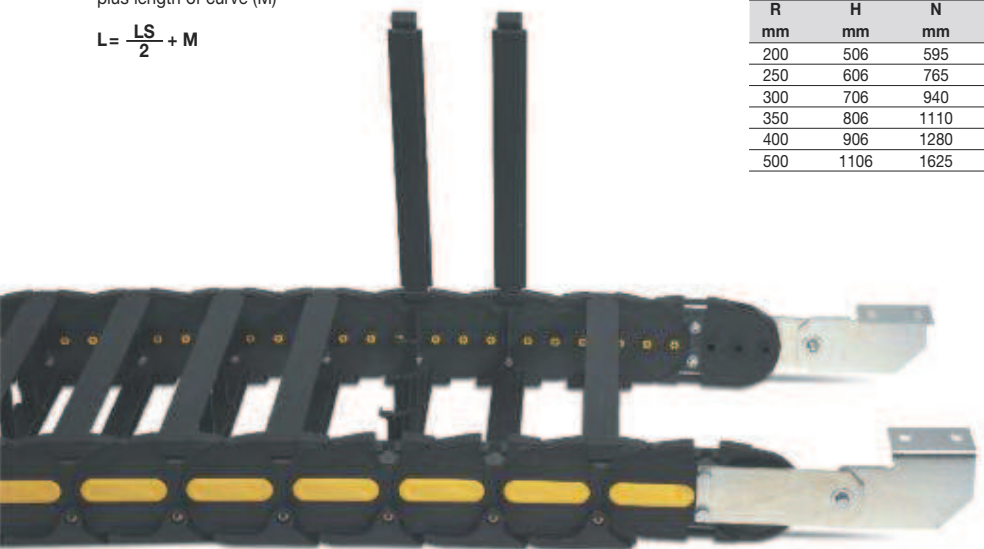
Version with frames mounted on every pitch.
