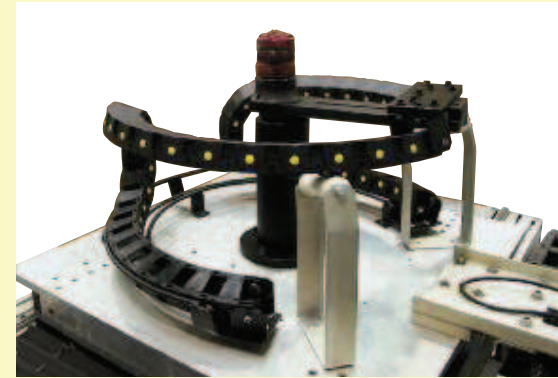
Support rollers view.
