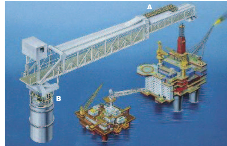
Platform "Oseberg"
