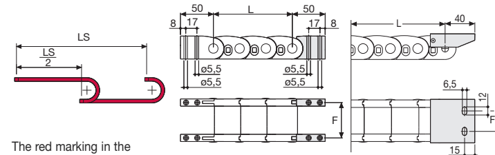
Fig. B Chain fixed outside the radius. (Fig B) See end brackets mounting variations page 31.
