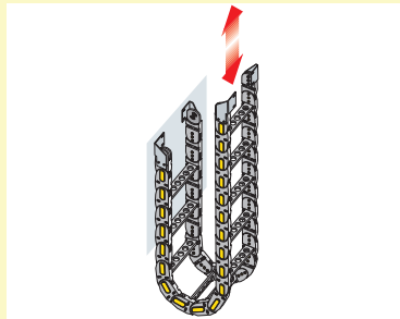
Vertical with curve below (see page 20).
