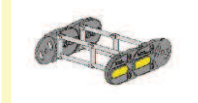
Aluminium rods screwed at the links. Maximum strength in every application. Possibilities in customising it's width. A separation of cables system.
