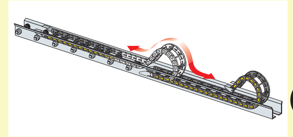
Long horizontal - 1 chain (see page 22).
